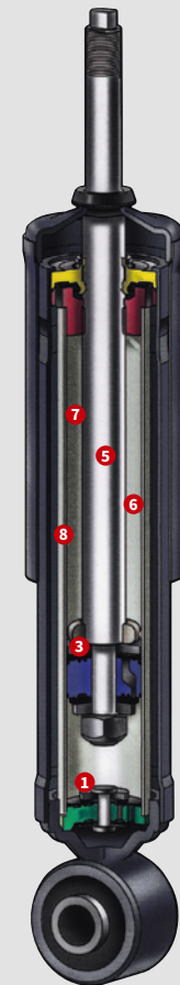
Conventional Shock Absorber
